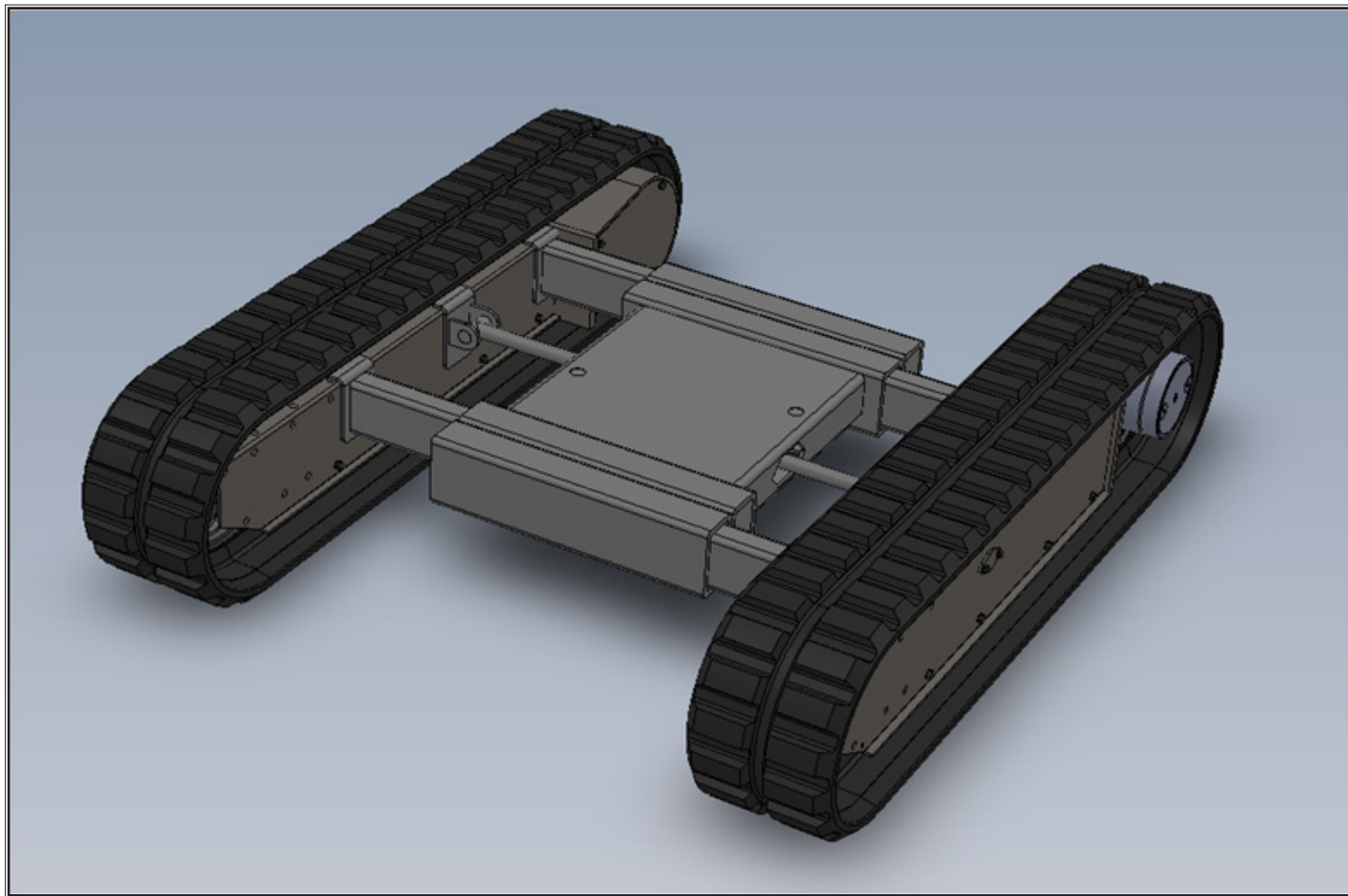
TRK40LT/TRK40/TRK60 TRACKS SYSTEMS OPTIONAL EXT EXPANDER
